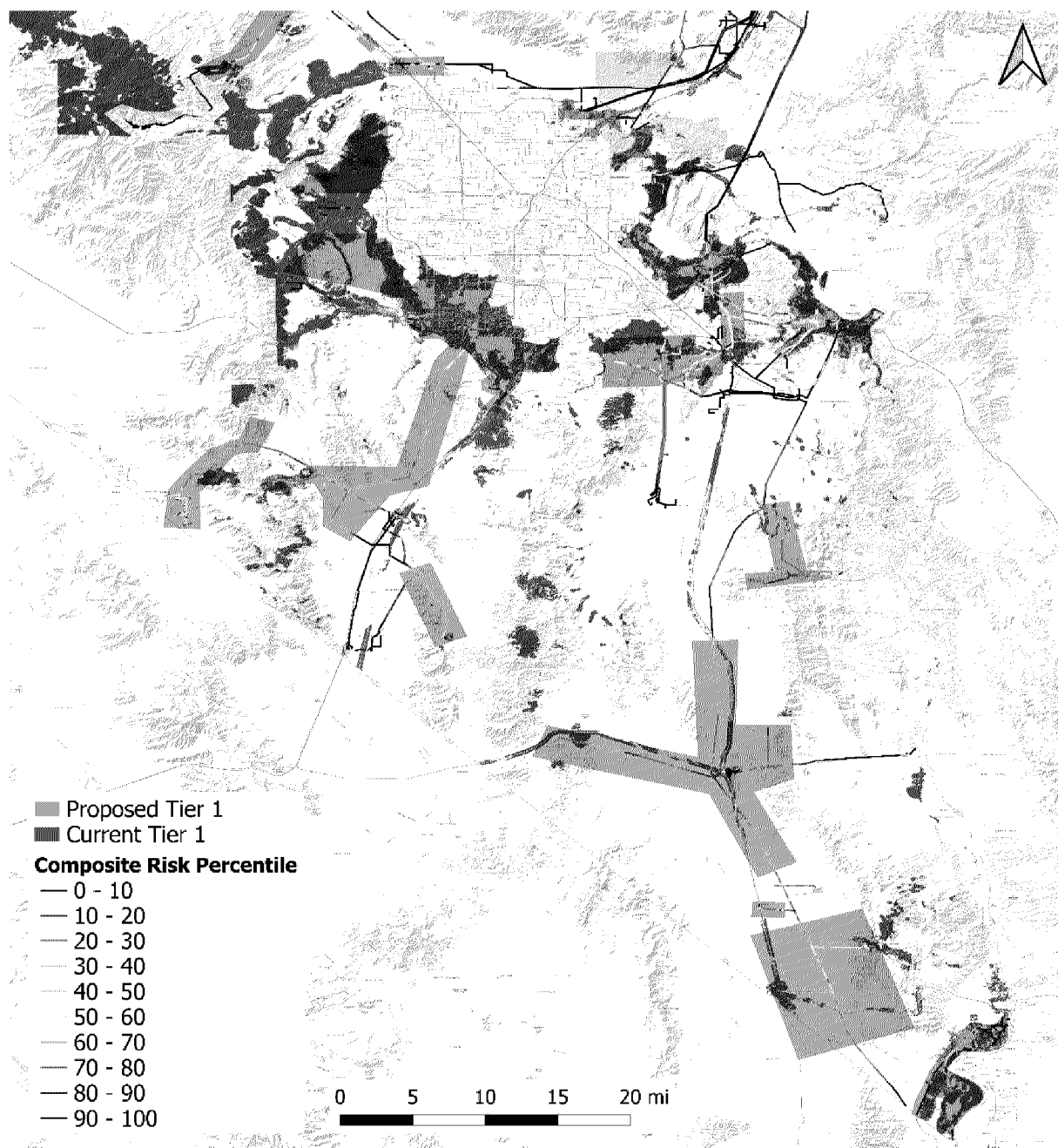
Figure 71. Proposed Tier 1 Refresh and Current Tier 1 in Southern Nevada
