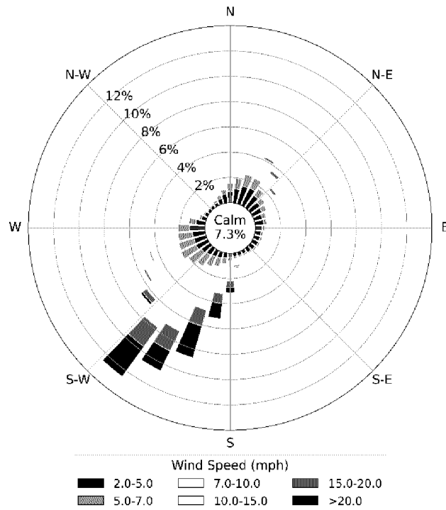
Figure 39. Sustained Wind Speeds at Tahoe-Donner RAWS
