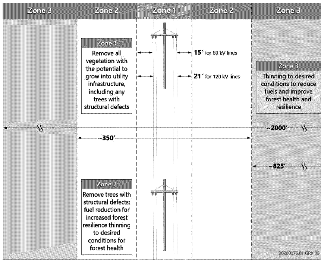
Figure 25. Resilient Corridors Clearance Example
