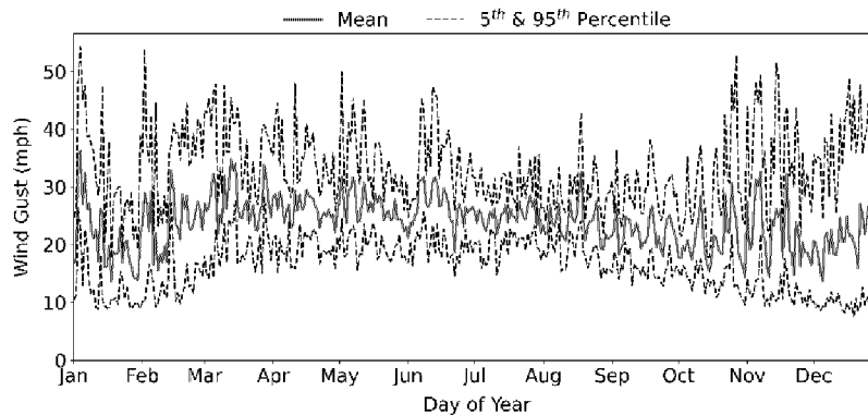
Figure 56. Climatology of Daily Maximum Wind Gust at NV005 Weather Station
