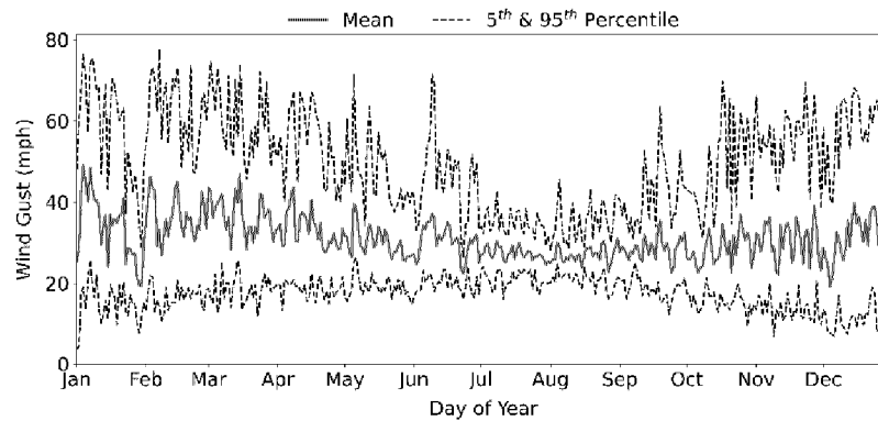
Figure 40. Climatology of Daily Maximum Wind Gust at Tahoe-Donner RAWS
