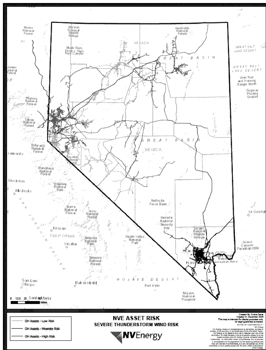
Figure 8. Thunderstorm Wind Risk
