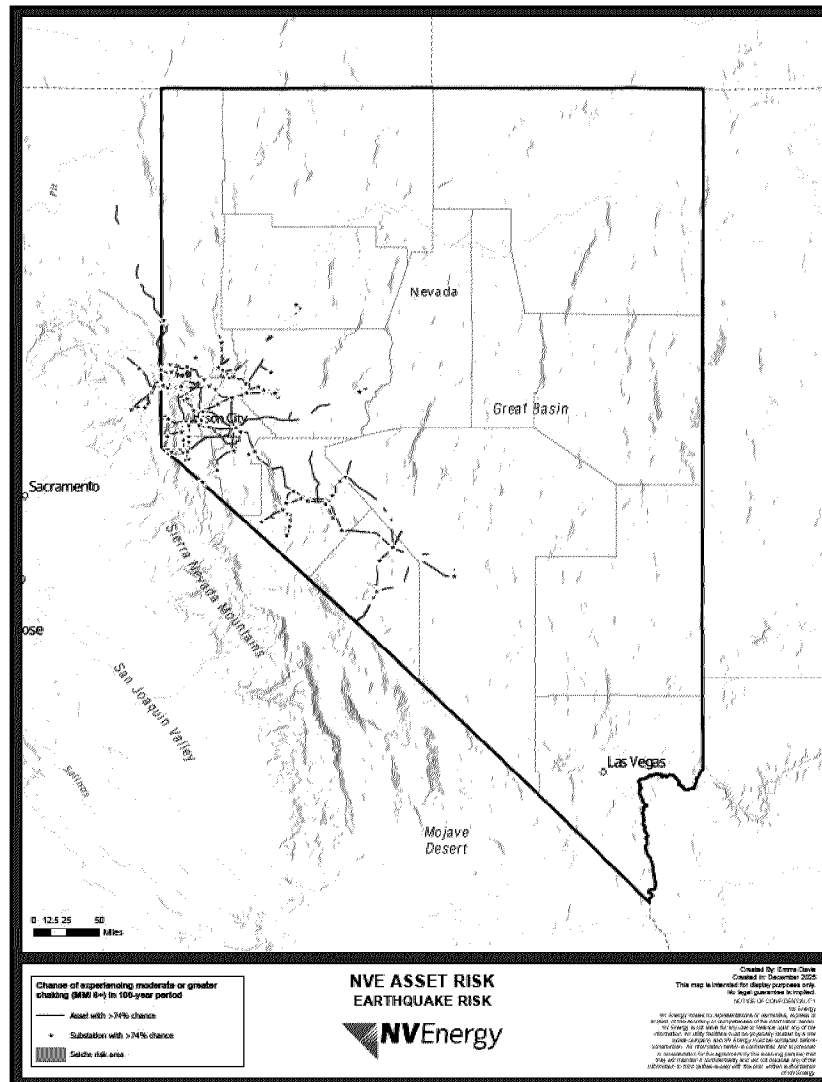
Figure 10. Earthquake Risk
