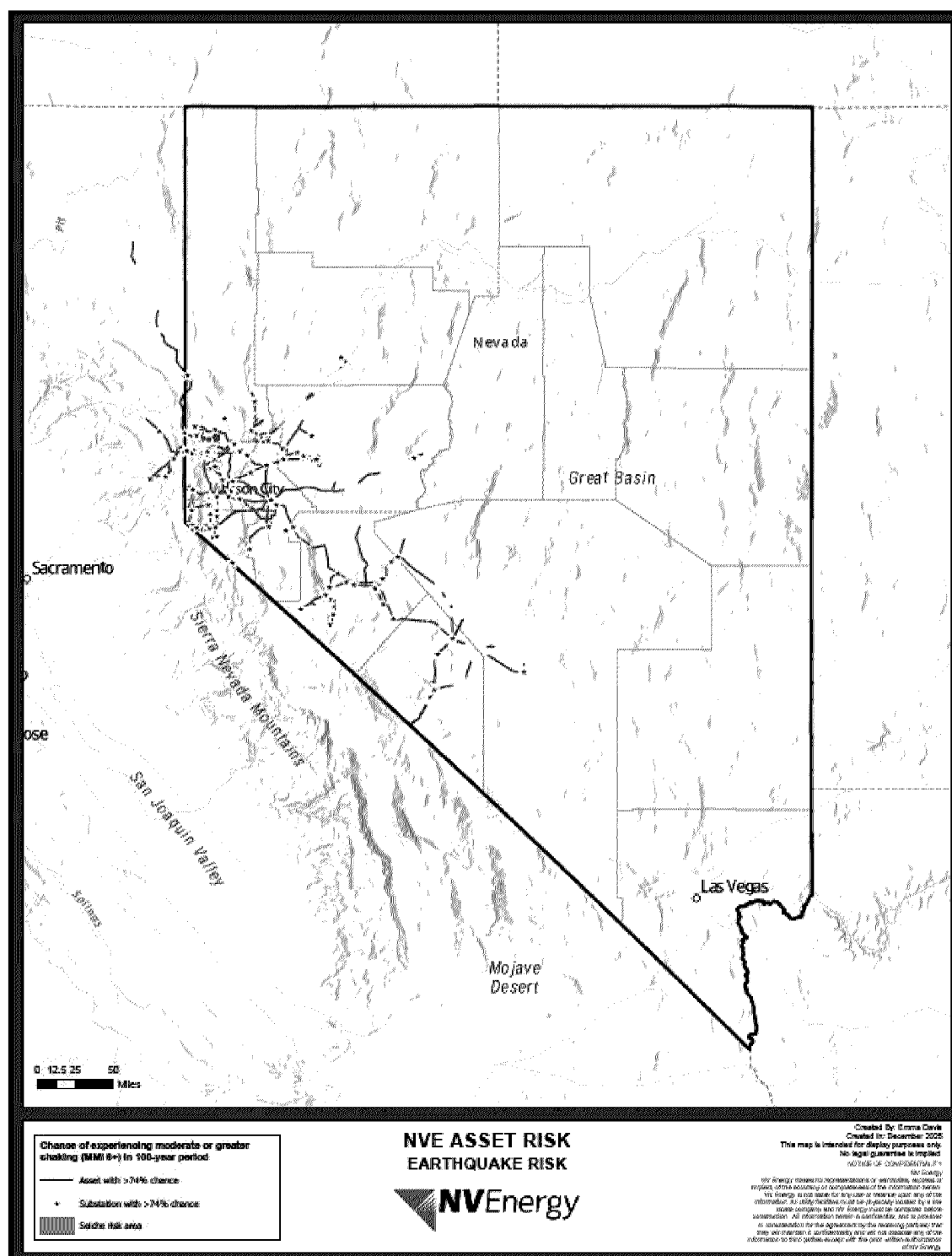
Figure 9. Earthquake Risk
