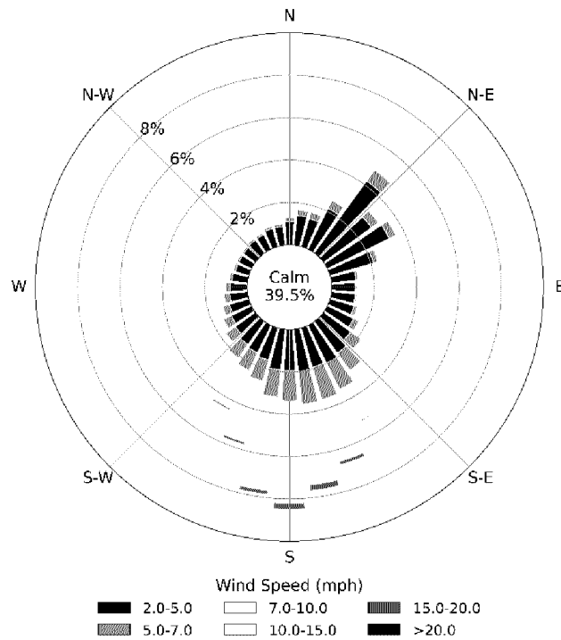
Figure 41. Sustained wind speeds at Tahoe-Donner RAWS
